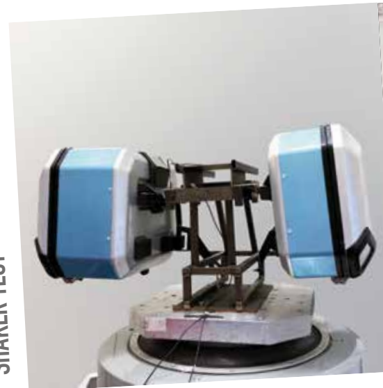
WEATHERING TEST
